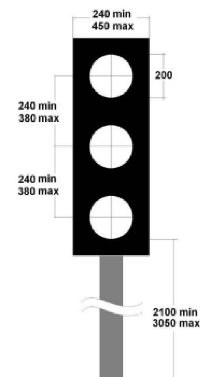
Figure 9.1: Dimensions of Standard Signal Head
